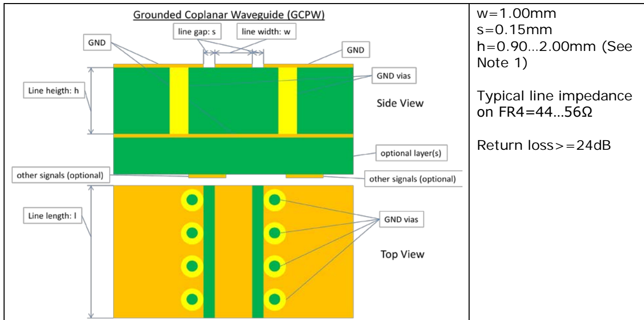
Figure 5 – Transmission line specification
