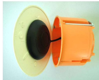
Figure: Mounting a Patch Antenna
