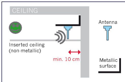
Figure: Mounting a Magnetic Antenna
