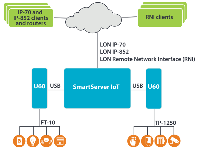
Use separate USB interface module for each channel
