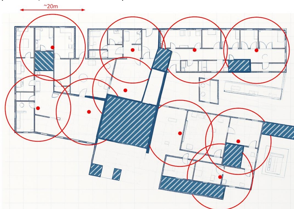
Figure 11: Coverage Circles on Floor Plan.
