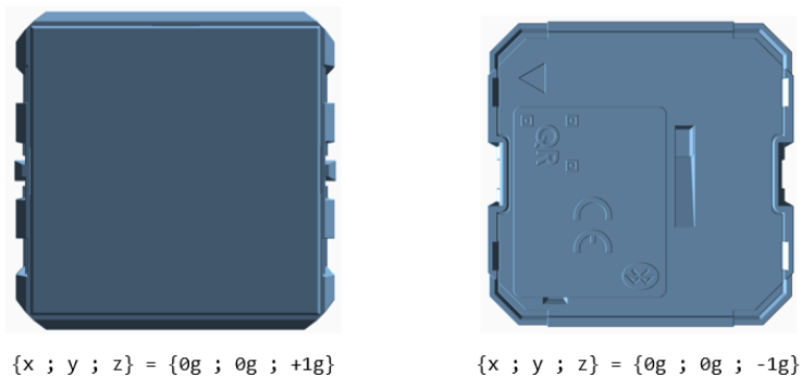
Figure 62 – Acceleration vector based on device orientation
