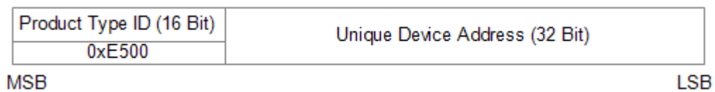
Figure 17 – BLE static source address structure
