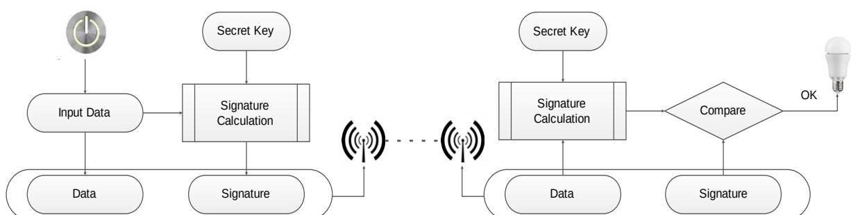
Figure 15 – Telegram authentication
