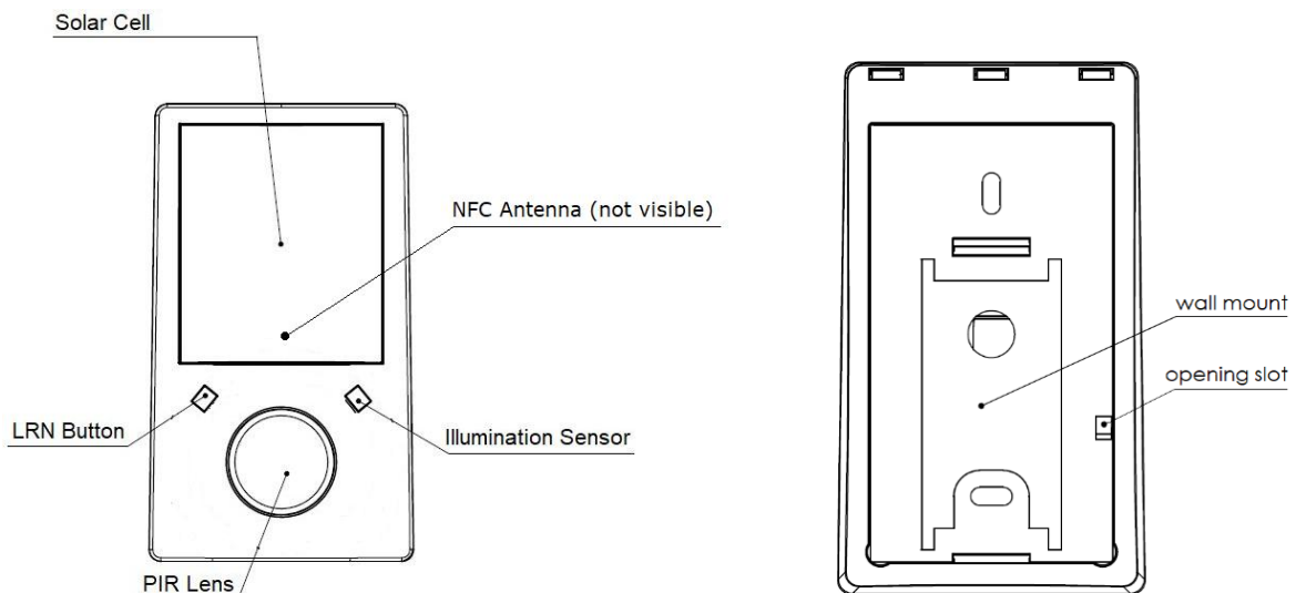
Figure 2 – EMDCB front and rear view
