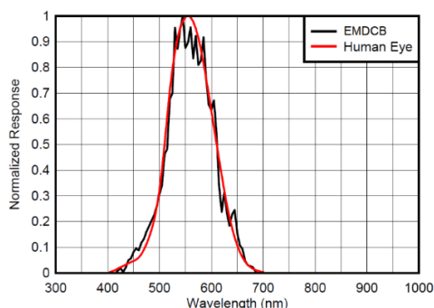
Figure 8 – Spectrum response of the ambient light sensor
