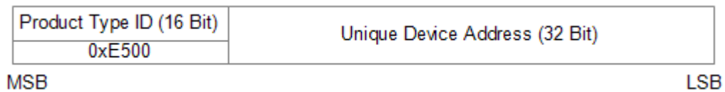
Figure 17 – BLE static source address structure
