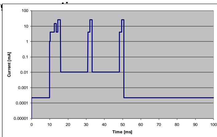
Current Consumption of STM 300x
