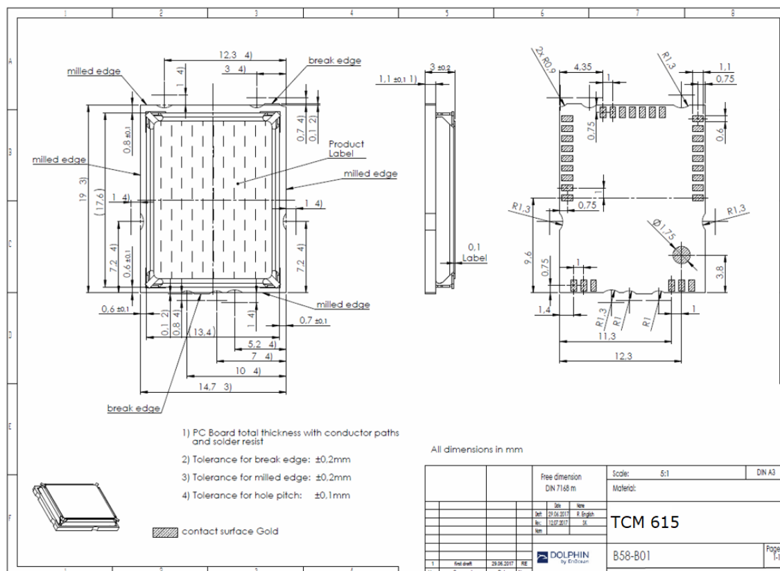
Figure 19 – Device outline
