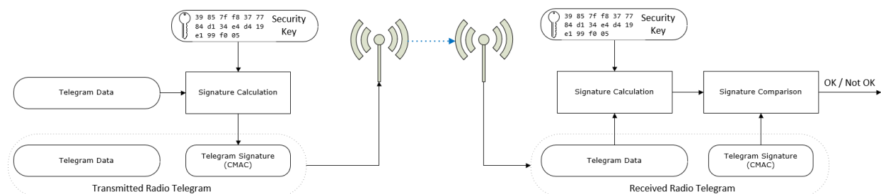
Figure 55 – Telegram authentication via telegram signature
