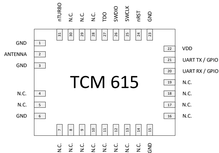
Figure 4 – TCM 615 device interface
