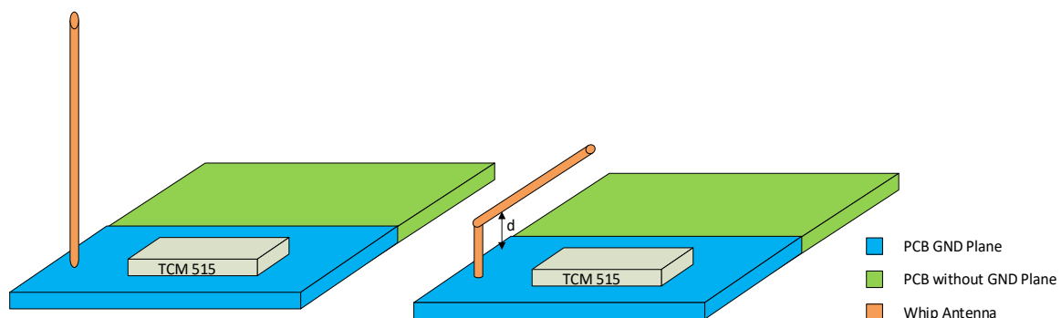
Figure 25 – Whip antenna positioning
