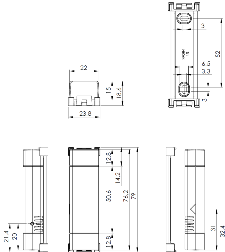
ETHSx Mechanical Outline (with mounting plate)
