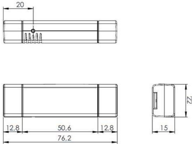
ETHSx Mechanical Outline (with 2 square caps, without stand)
