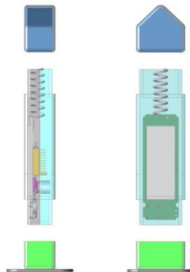
ETHSx Mechanical Outline (with triangle cap and stand)
