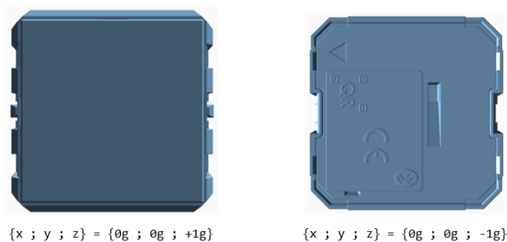
Figure 69 – Acceleration vector based on device orientation
