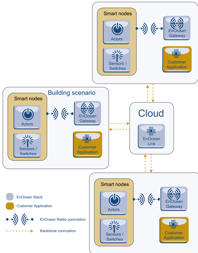
Figure 2 EnOcean Link in the Cloud
