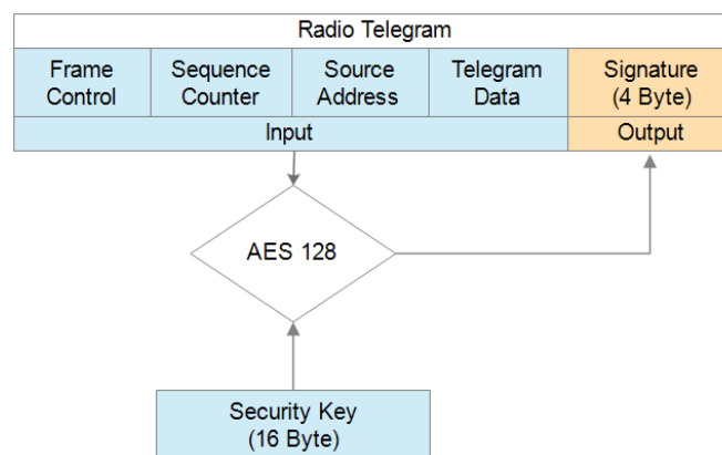
Figure 7 – Data telegram authentication flow
